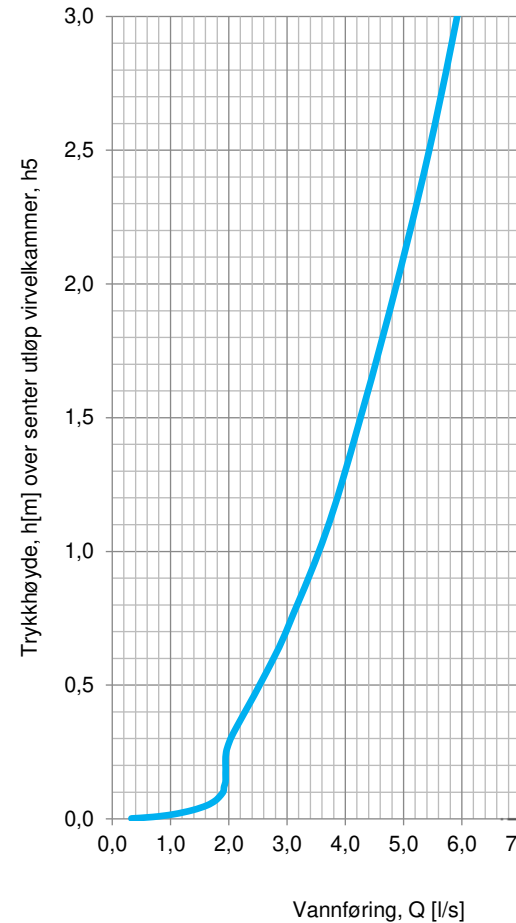
Hydraulisk kurve
