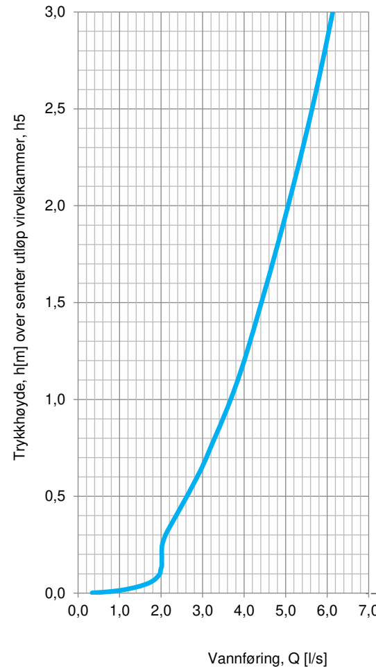
Hydraulisk kurve
