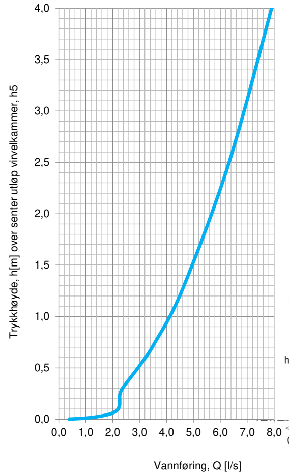
Hydraulisk kurve
