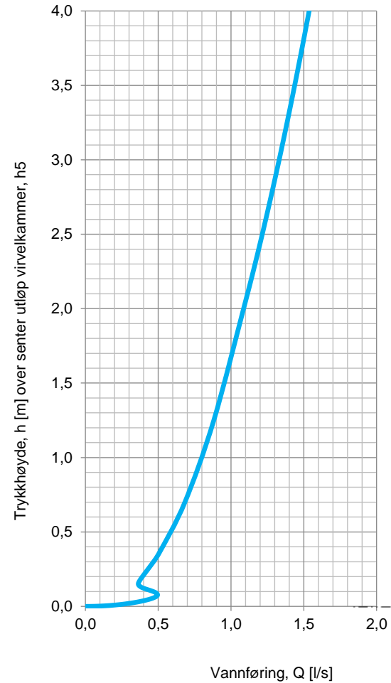
Hydraulisk kurve
