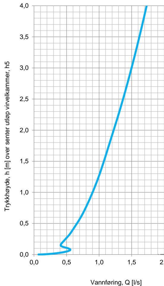
Hydraulisk kurve
