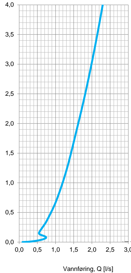
Hydraulisk kurve
