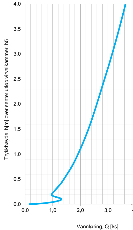
Hydraulisk kurve
