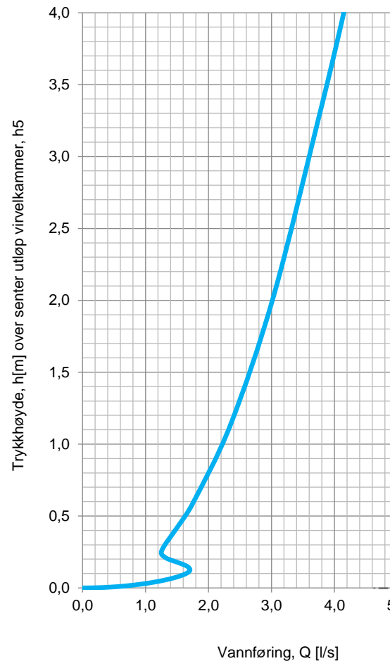
Hydraulisk kurve
