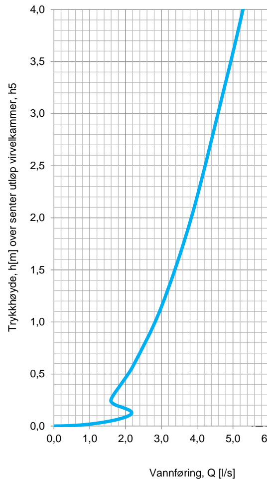
Hydraulisk kurve
