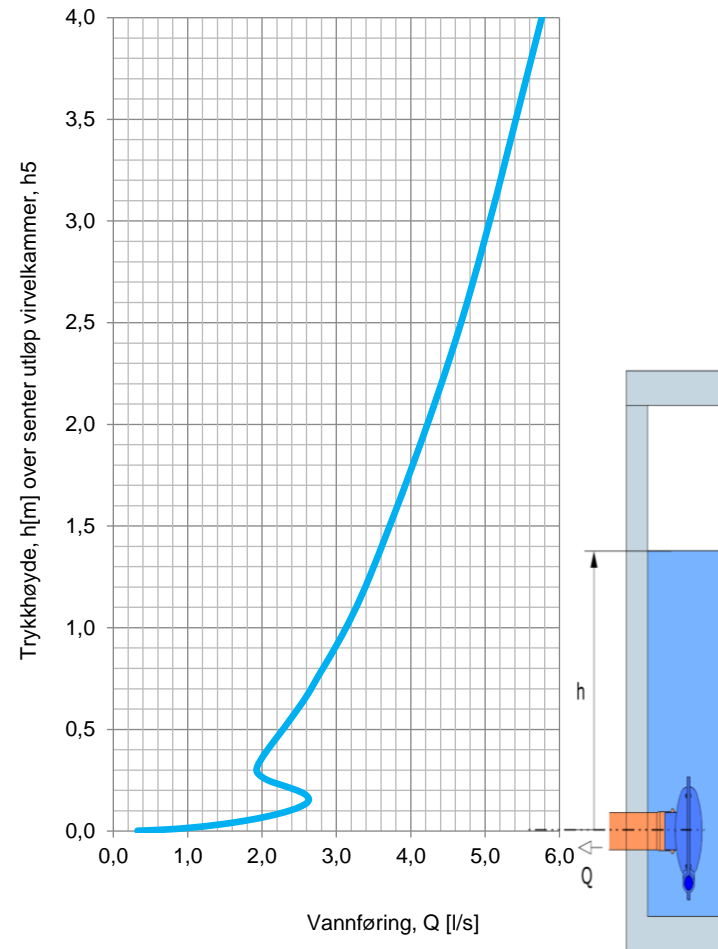
Hydraulisk kurve
