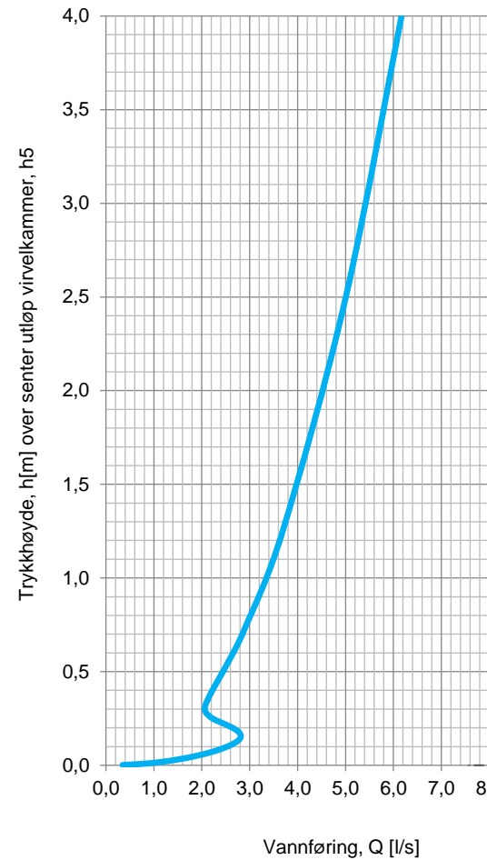
Hydraulisk kurve
