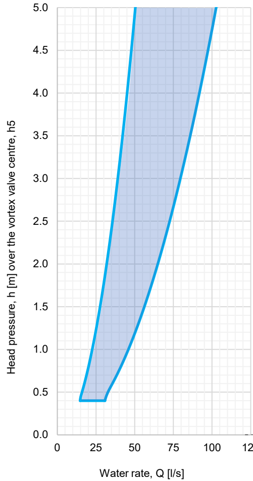
Recommended Hydraulic Dimensioning Range
