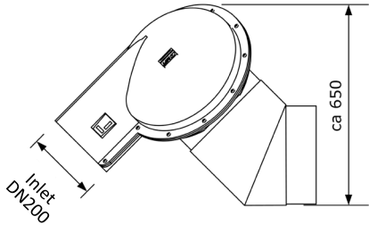
Type P2 with mounting plate
