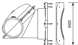
Type P1 with mounting plate
