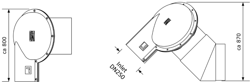
Type P1 with mounting plate
