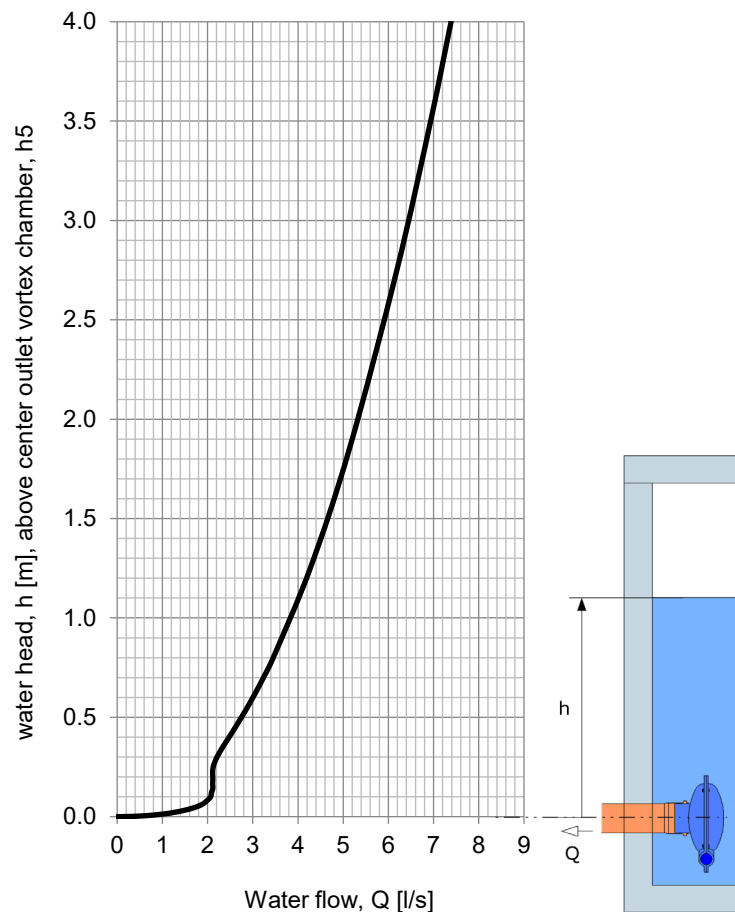
Hydraulic curve
