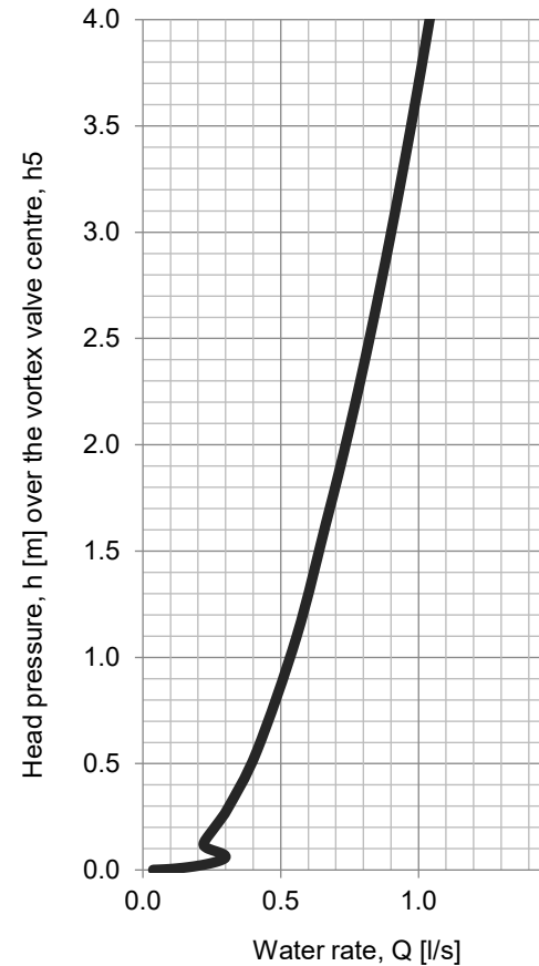
Hydraulic curve
