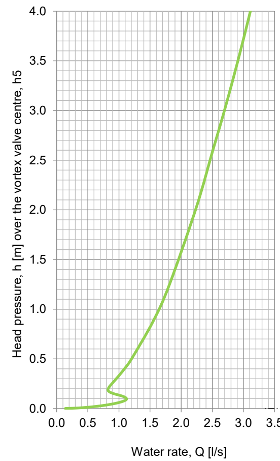
Hydraulic curve
