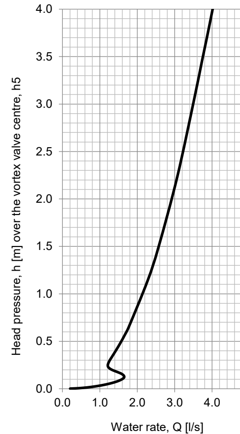
Hydraulic curve
