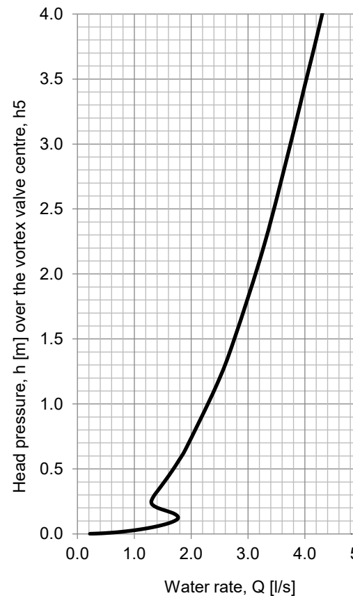
Hydraulic curve
