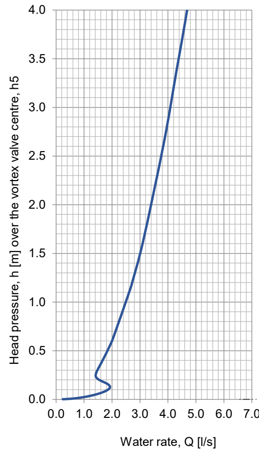
Hydraulic curve
